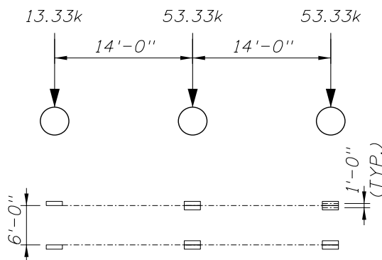
FL120 Permit Vehicle GVW = 120k
